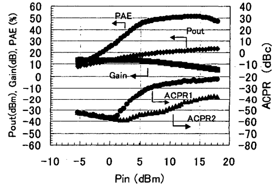
Fig.4. Output power, power gain, power-added-efficiency and ACPR versus input power for the HBT with 0.75 \mu\text{m} collector layer thickness and slightly doping SiC structure • • at 1.95 GHz, V_{\text{CE}} = 2.7\text{V} .
